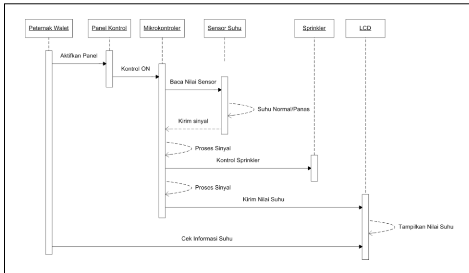
Gambar 4. Sequence Diagram Pengontrolan Suhu
